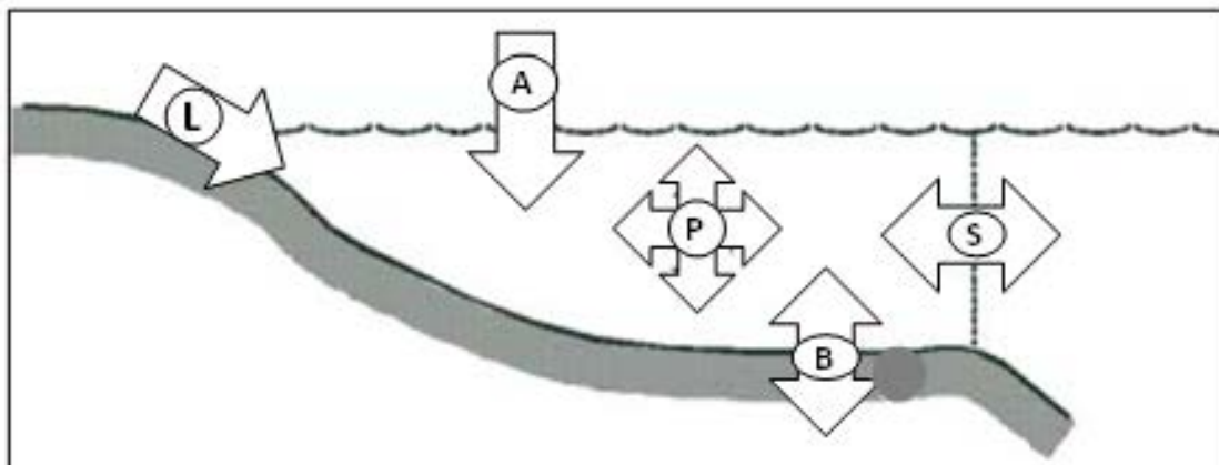
Figure 5. A schematic of pressures and interactions that govern coastal ecosystem states and state changes. Pressures include land-based inputs (L); net atmospheric inputs (A); and oceanic influences (S). Within coastal ecosystems, interactions between benthic and pelagic systems (B) and interactions within the pelagic environment (P) are influenced by pressures that lead to changes in states. Not shown are interactions among coastal ecosystems that propagate along the coast.
