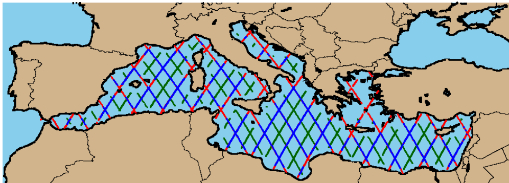
Figure 9. The hardware design and algorithm improvements for the Jason-2 Advanced Microwave Radiometer (AMR) have greatly improved coastal sea level monitoring over its predecessor altimetry missions, Jason-1 and TOPEX/Poseidon. In particular, the spatial resolution of the wet troposphere correction derived from radiometer observations has nearly doubled. The coverage of the Jason-1/TOPEX references missions was limited to areas greater than 50 km from coasts and islands (blue), while Jason-2 additionally covers areas up to 26 km away (red dots). In 2009 Jason-1 was maneuvered into a ground track interleaved with Jason-2, and this coverage area is in green. Note that the AMR from Jason-2 is more important than the interleaved phase in providing coverage of the Adriatic and Aegean Seas. Courtesy of the NOAA Laboratory for Satellite Altimetry.
